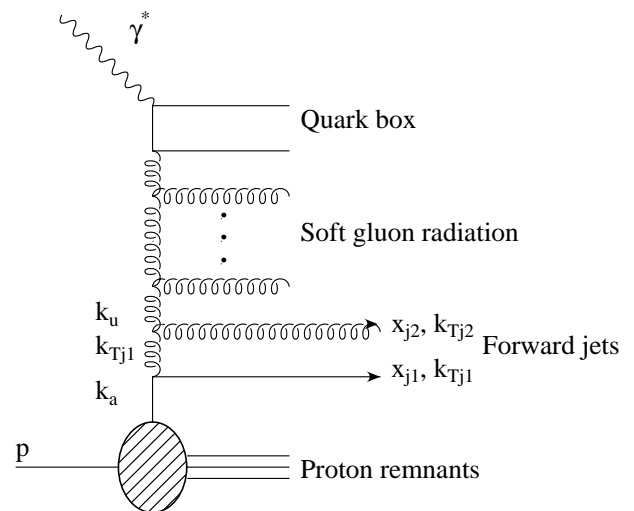
Fig. 11. Diagram illustrating the emission of an extra forward jet in addition to the standard Mueller process
