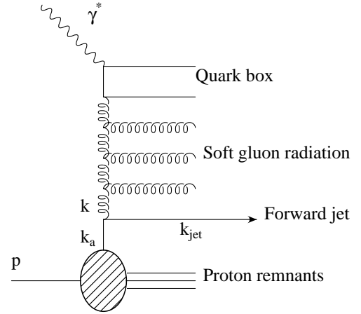
Fig. 3. Diagram showing forward jet production driven by \gamma^* g fusion coupled to evolution through a BFKL-type ladder. The struck parton from the proton could in principle be either a gluon or a quark
