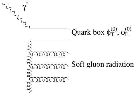
Fig. 1. Diagram showing the \gamma^*g fusion, including the soft gluon radiation ladder
