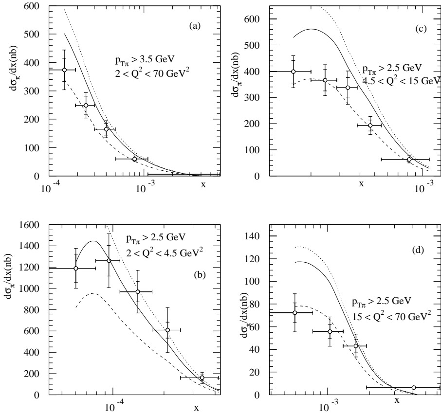
Fig. 7. The \pi^0 differential cross-section versus Bjorken- x obtained from 1996 H1 (preliminary) data [12]. The curves are predictions, based on the BFKL formalism including sub-leading corrections, corresponding to the three choices of scales and infrared cut-off given in (13)
