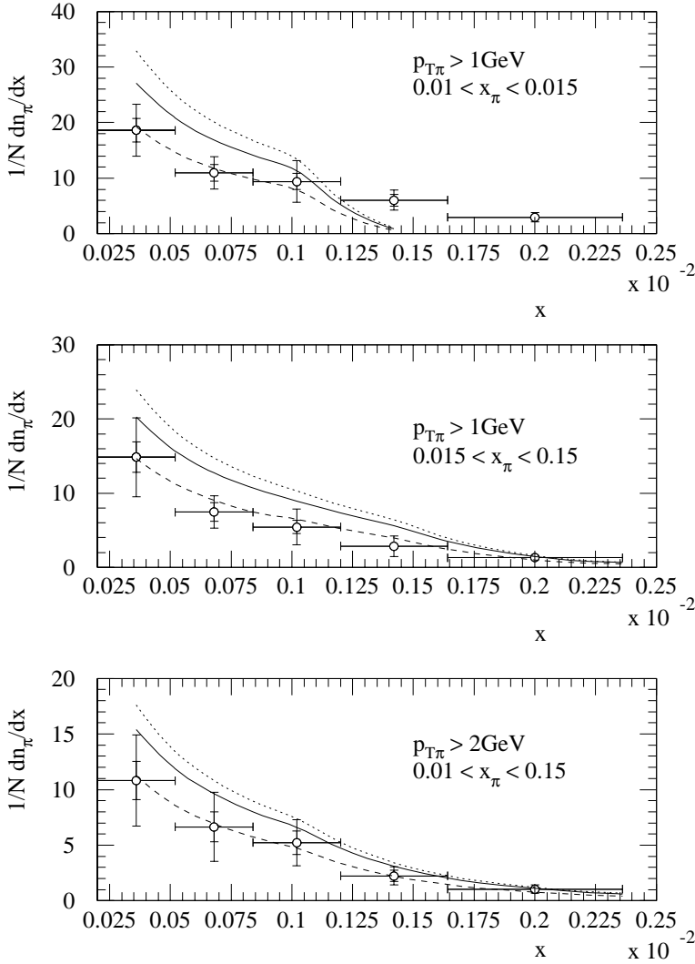
Fig. 6. The \pi^0 spectra (16) versus Bjorken- x obtained from 1994 H1 data [10]. The curves are predictions, based on the BFKL formalism including sub-leading corrections, corresponding to the three choices of scales and infrared cut-off given in (13). [The restriction x/x_\pi < 0.1 limits the comparison to the domain x \lesssim 10^{-3} in the upper plot.]
