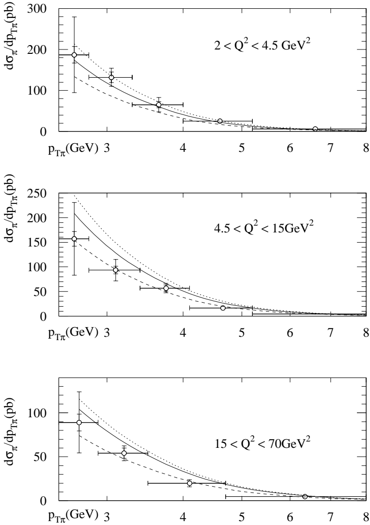
Fig. 8. \pi^0 differential cross-section in transverse momentum, obtained from 1996 H1 (preliminary) data [12]. The curves are predictions, based on the BFKL formalism including sub-leading corrections, corresponding to the three choices of scales and infrared cut-off given in (13)
