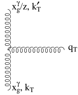
Fig. 2. Diagram to illustrate the radiation of soft gluons from the reggeized gluonic propagator in the t -channel
