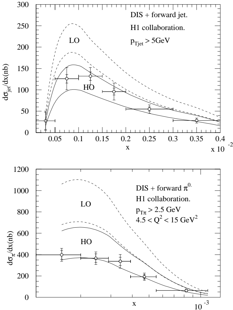
Fig. 12. The differential cross-section for a DIS + forward jet, b DIS + forward \pi^0 (1996 H1 preliminary), events. The continuous and dashed curves correspond to the inclusion and omission of the consistency constraint. The lower curve of each pair corresponds to choosing the scales of \alpha_S in (4) and (10) to be k_T^2 + m_q^2 and k_T^2 respectively. The upper curves have scales 1/4 of these values. In all cases the infrared cut-off in (7) is taken to be k_0^2 = 0.5 \text{ GeV}^2 . The jet data are at the hadron level; converting to the parton level is expected to lower the jet data points by about 15-20% [17]
