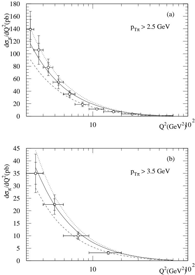
Fig. 9. The \pi^0 differential cross-section versus Q^2 obtained from 1996 H1 (preliminary) data [12]. The curves are predictions, based on the BFKL formalism including sub-leading corrections, corresponding to the three choices of scales and infrared cut-off given in (13)
