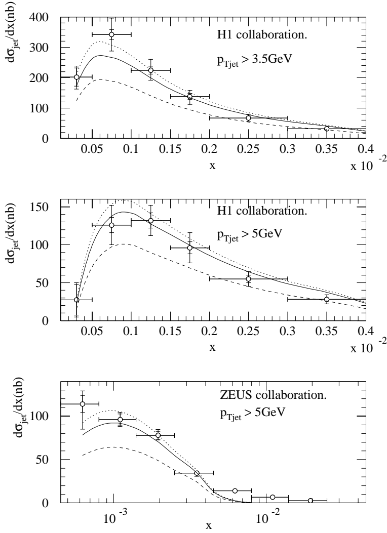
Fig. 4. The DIS + forward jet differential cross-section versus Bjorken- x as measured at the hadron level by the H1 [10] and ZEUS [11] collaborations. The kinematic cuts are given in Table 1. The curves are predictions at the parton level, based on the BFKL formalism including sub-leading corrections, corresponding to the three choices of scales and infrared cut-off given in (13)
