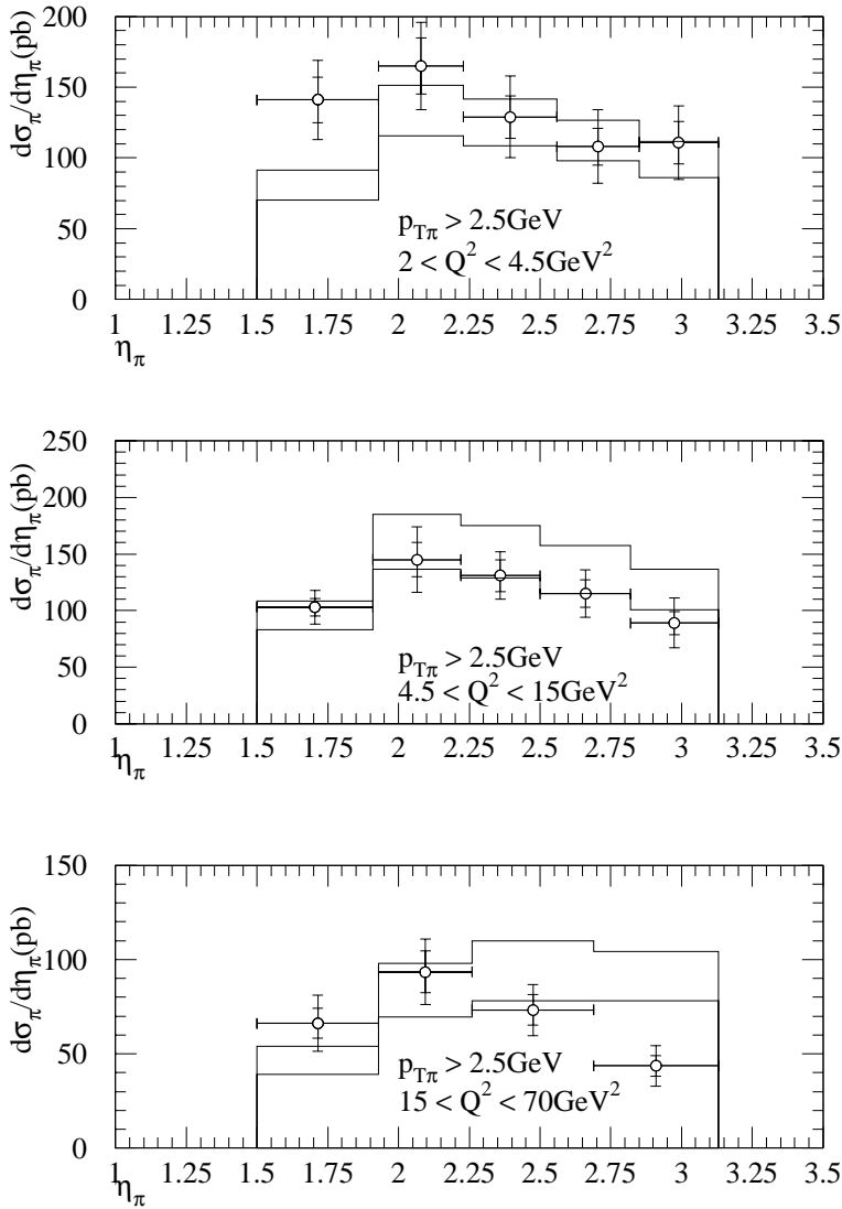
Fig. 10. The \pi^0 differential cross-section versus rapidity obtained from 1996 H1 (preliminary) data [12]. The upper and lower histograms are the predictions of the BFKL formalism including subleading corrections respectively corresponding to choices (ii) and (iii) of the scales and k_0^2 given in (13)
